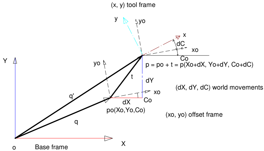
Figure 6: World coordinate move in the X-Y plane
