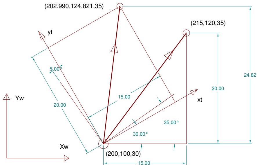
Figure 8: World and tool coordinate move in the X-Y plane
