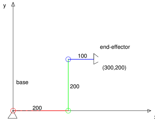
Figure 3: Example 1: Planer 3-dof serial arm
