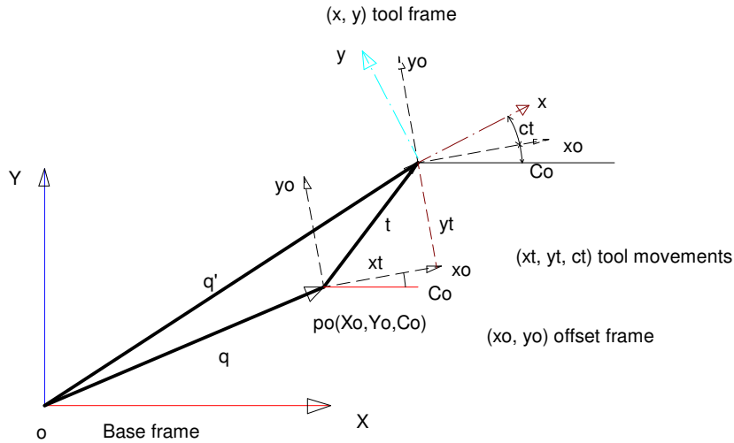
Figure 7: Tool coordinate move in the X-Y plane
