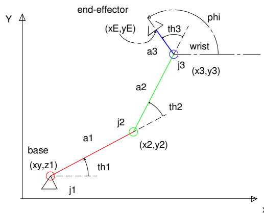
Figure 1: Planer 3-dof serial arm
