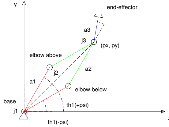
Figure 5: Two possible solutions for \theta_1
