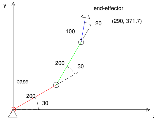
Figure 4: Example 2: Planer 3-dof serial arm
