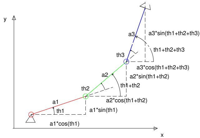
Figure 2: x- and y-components of links
